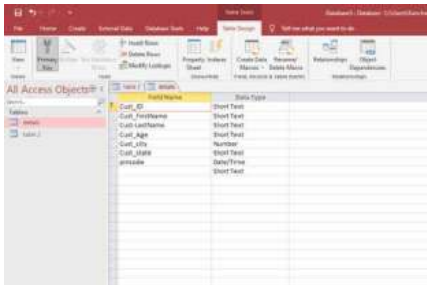
Figure 2.6: Primary Key
